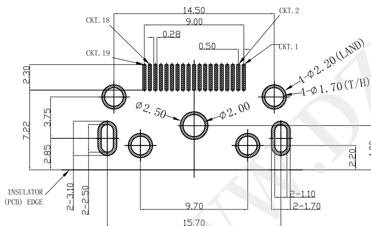
PCB PATTERN LAYOUT (T1.2±0.15)
